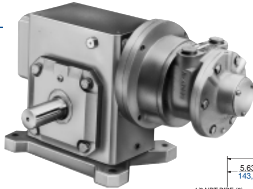
“B” Mounting (photo) 6AM-22A-CB10 (standard shaft) / *6AM-22A-CF10 (opposite shaft) inches / mm
