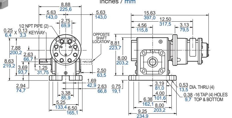
“B” Mounting (photo) 6AM-22A-CB10 (standard shaft) / *6AM-22A-CF10 (opposite shaft) inches / mm
