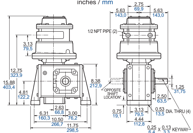
6AM-22A-CD10 (standard shaft) / *6AM-22A-CH10 (opposite shaft) inches / mm
