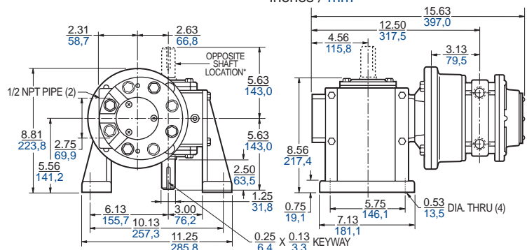
6AM-22A-CC10 (standard shaft) / *6AM-22A-CG10 (opposite shaft) inches / mm
